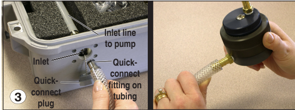
Unscrew the quick-connect plug. Use tubing with a quick-connect fitting to attach the case (pump) inlet to the outlet of impactor.
