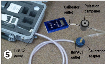
Use a short length of calibration tubing to connect inlet of calibration adapter to outlet of a calibrator to form a calibration train. Note: SKC High Flow chek-mate Calibrator requires Pulsation Dampener Cat. No. 375-150 in line as shown at above right and in Step 5 photo (see Accessories).
