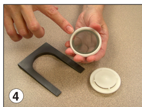
Ensure the stainless steel support screen is in place in the bottom of the filter cassette.
